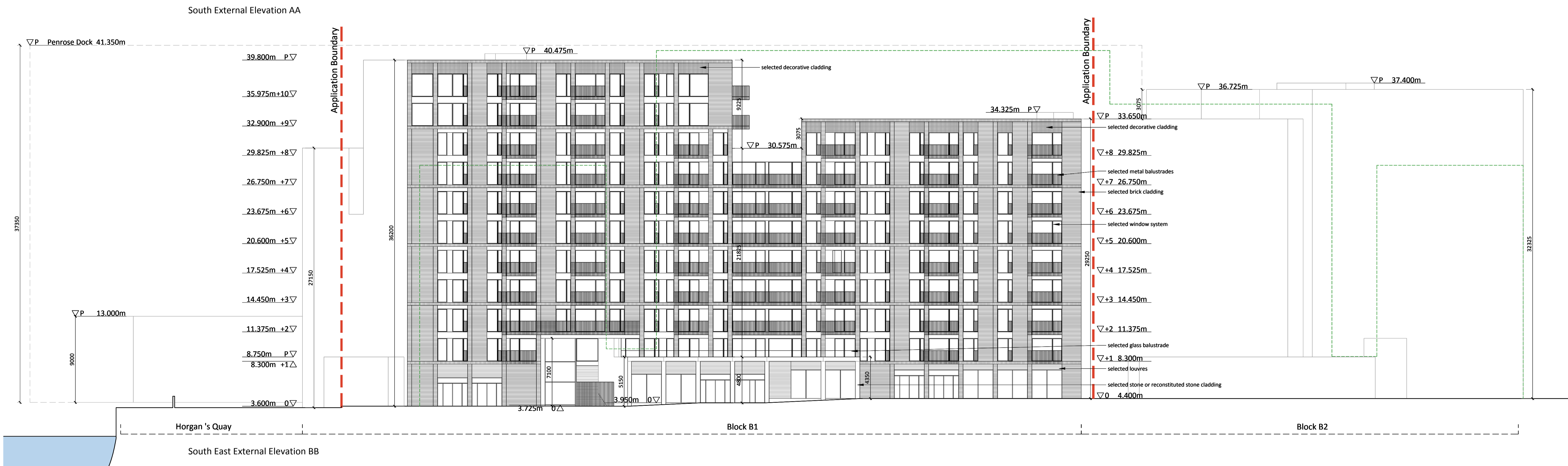
Elevations AA & BB
