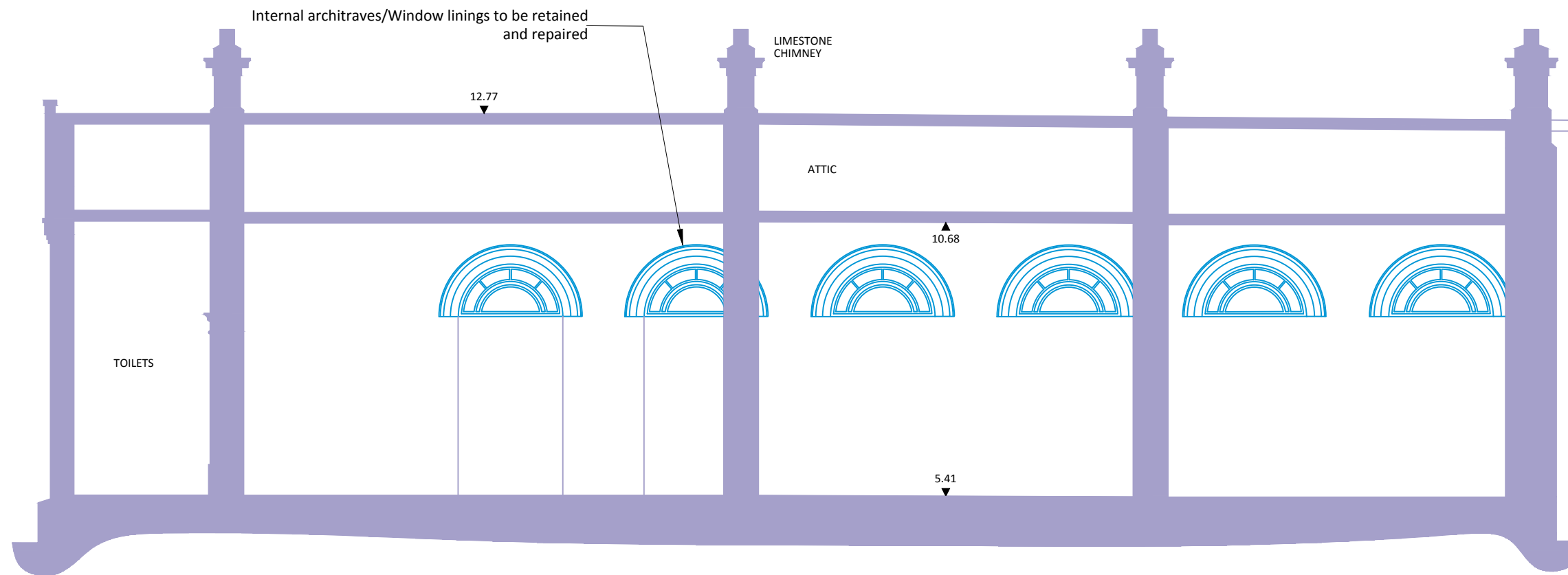
Section 1-1 - Existing
