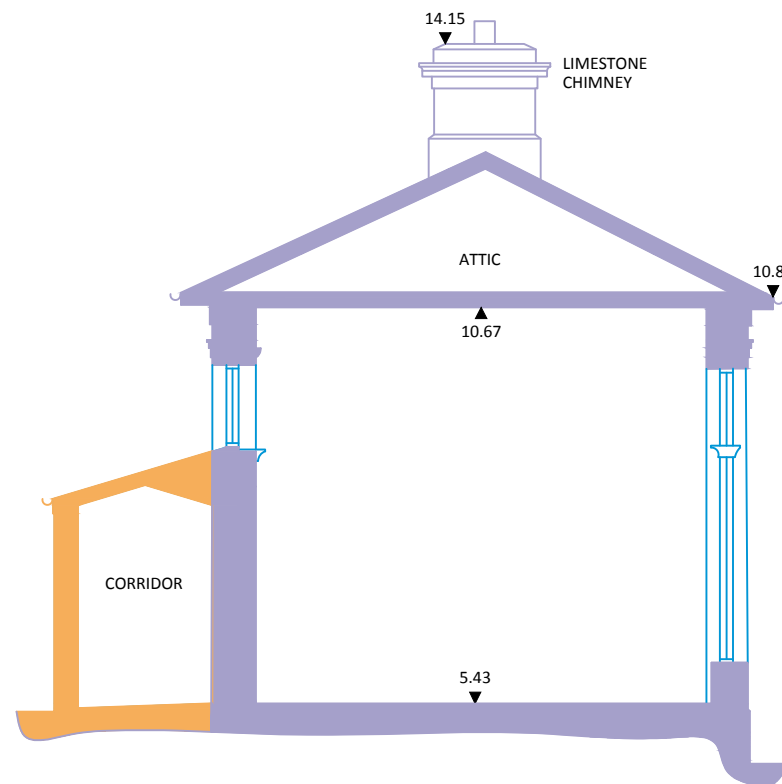
Section 2-2 - Existing
