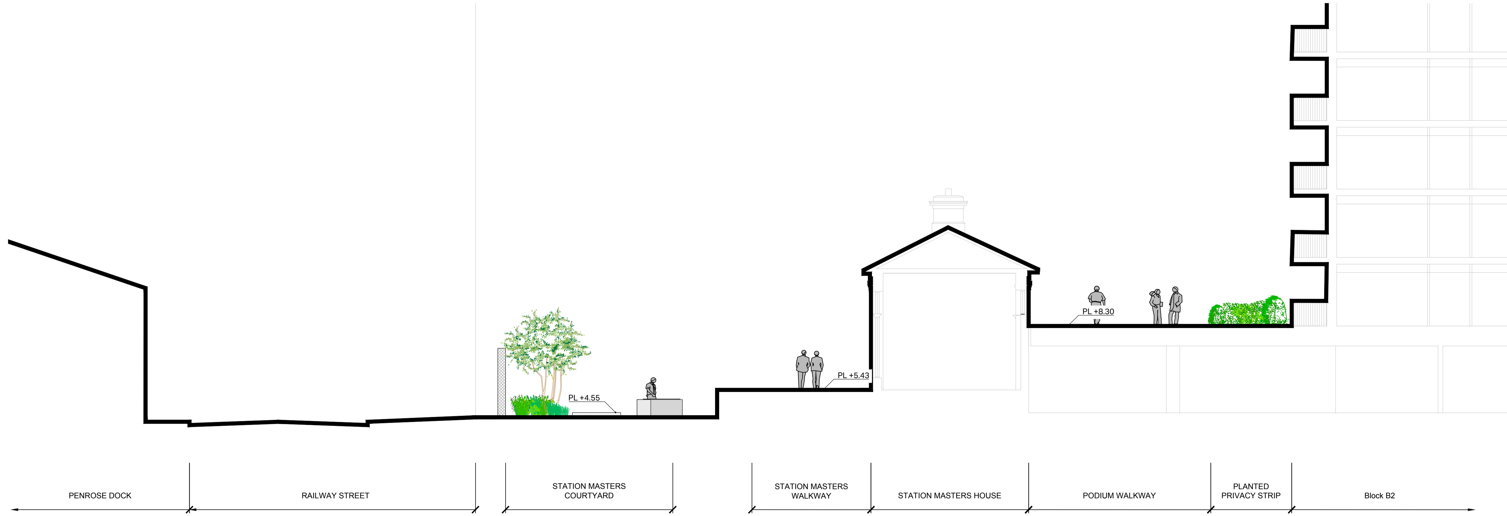
A SECTION A - A 6000 Scale 1:200
