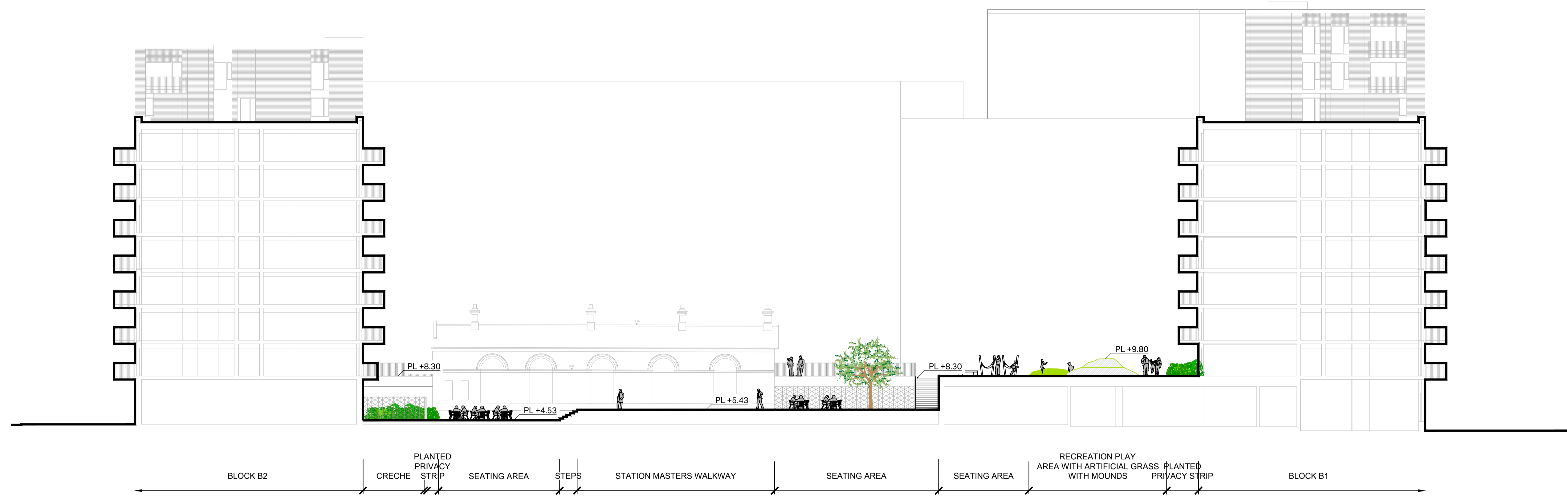
A SECTION A - A 6000 Scale 1:200
